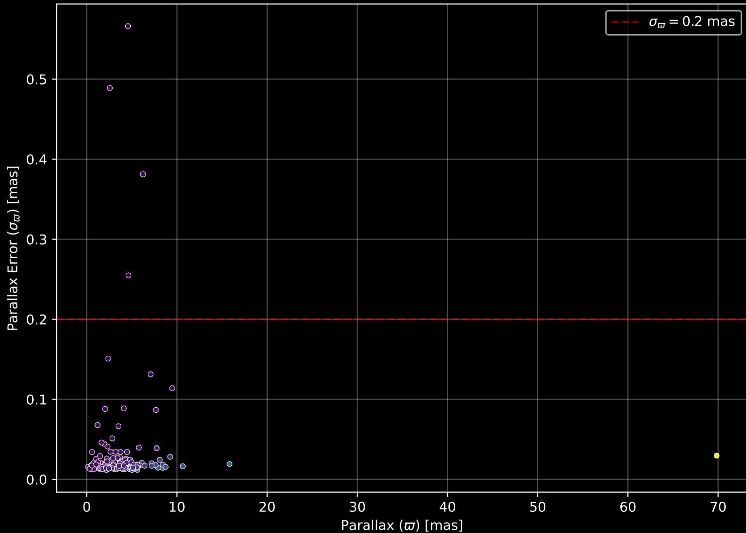
APOGEE DR17 Field: [130+74_MGA] Parallax Quality (n= 186)
