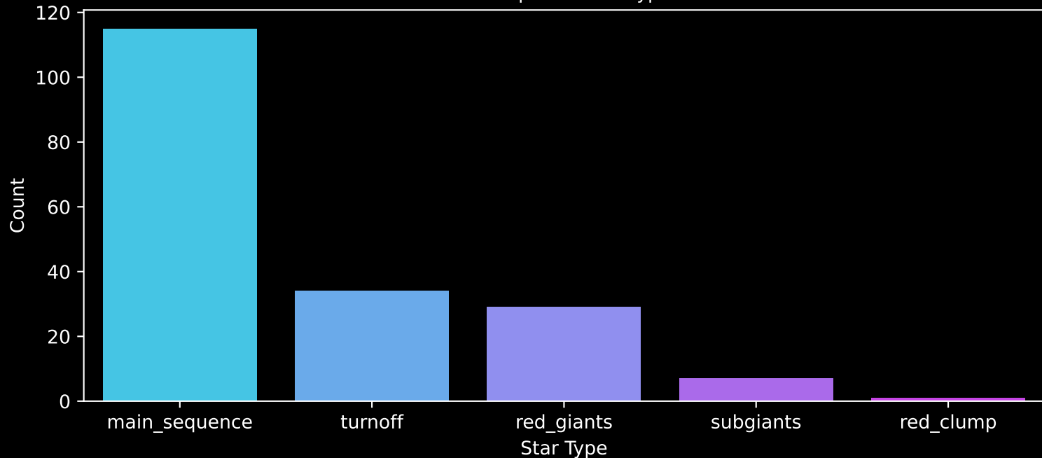
APOGEE DR17 Field: [130+74_MGA] Count plot of Star Type
