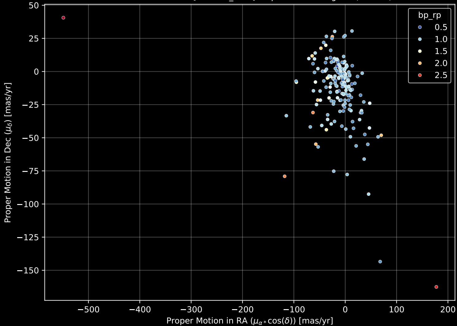
APOGEE DR17 Field: [130+74_MGA] Proper Motion Diagram (n= 186)
