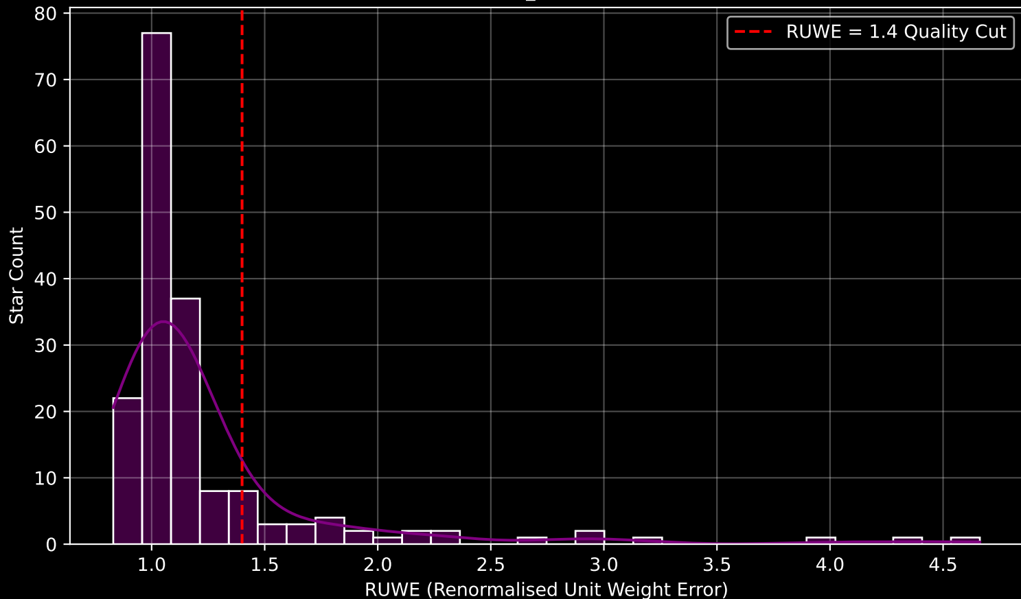
GAPOGEE DR17 Field [130+74_MGA] RUWE Distribution (n= 176)
