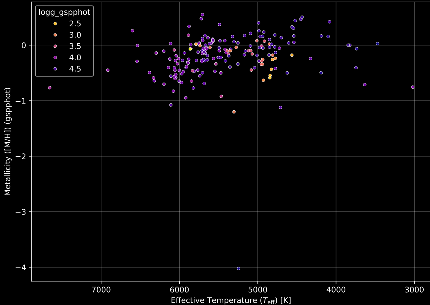
APOGEE DR17 Field: [130+74_MGA] Stellar Population Parameters (n= 186)
