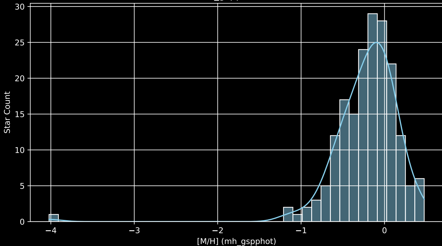
APOGEE DR17 Field: [130+74_MGA [M/H] (mh_gspphot) (n= 184)
