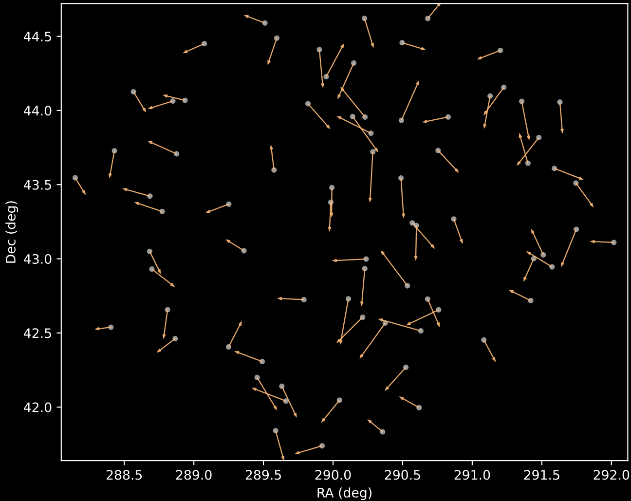
APOGEE DR17 Cluster 3 Proper Motion Vectors (n=76)
